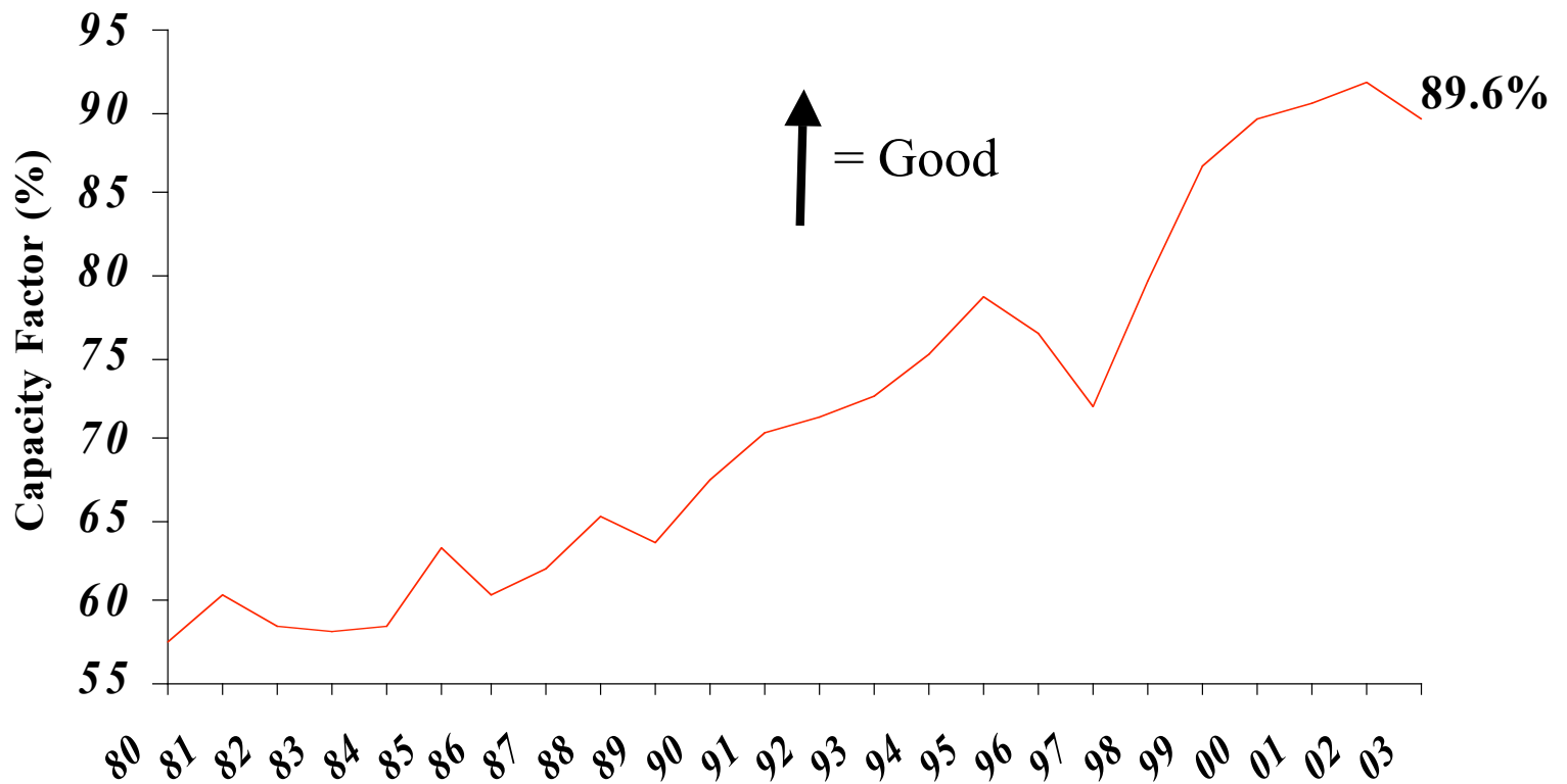
Capacity Factor of U.S. Nuclear Plants 1980-2003
